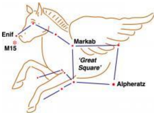
Pegasus, the flying horse
