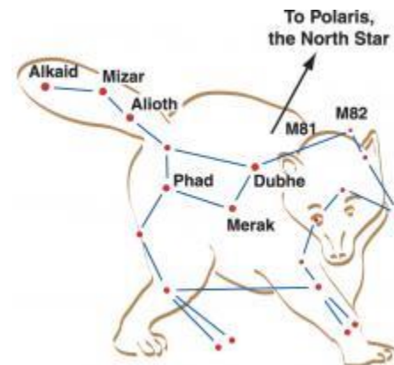
Ursa Major, (contains the big dipper)
