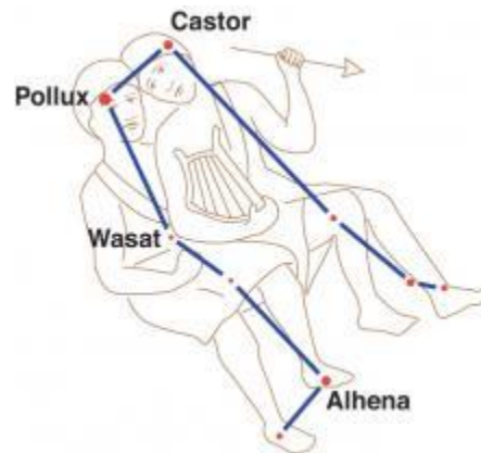
Gemini, the Twins
