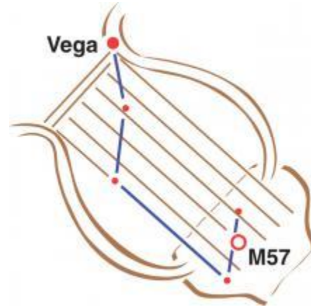
Lyra, the harp
