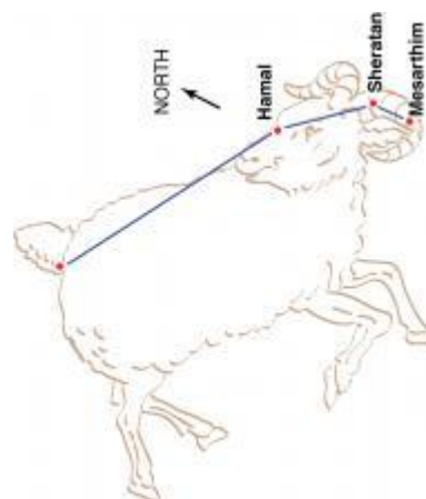
Aries, the Ram
