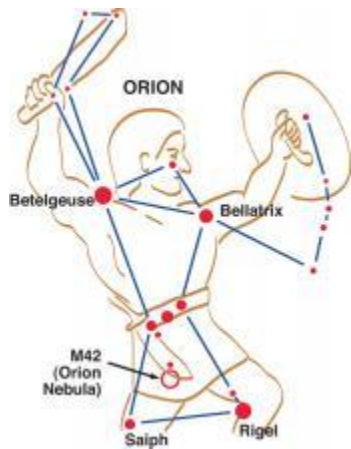
Orion, The hunter
