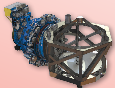
SOFIA telescope
