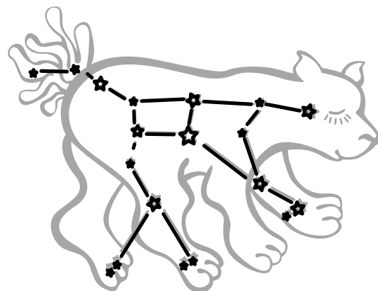
Ursa Major
